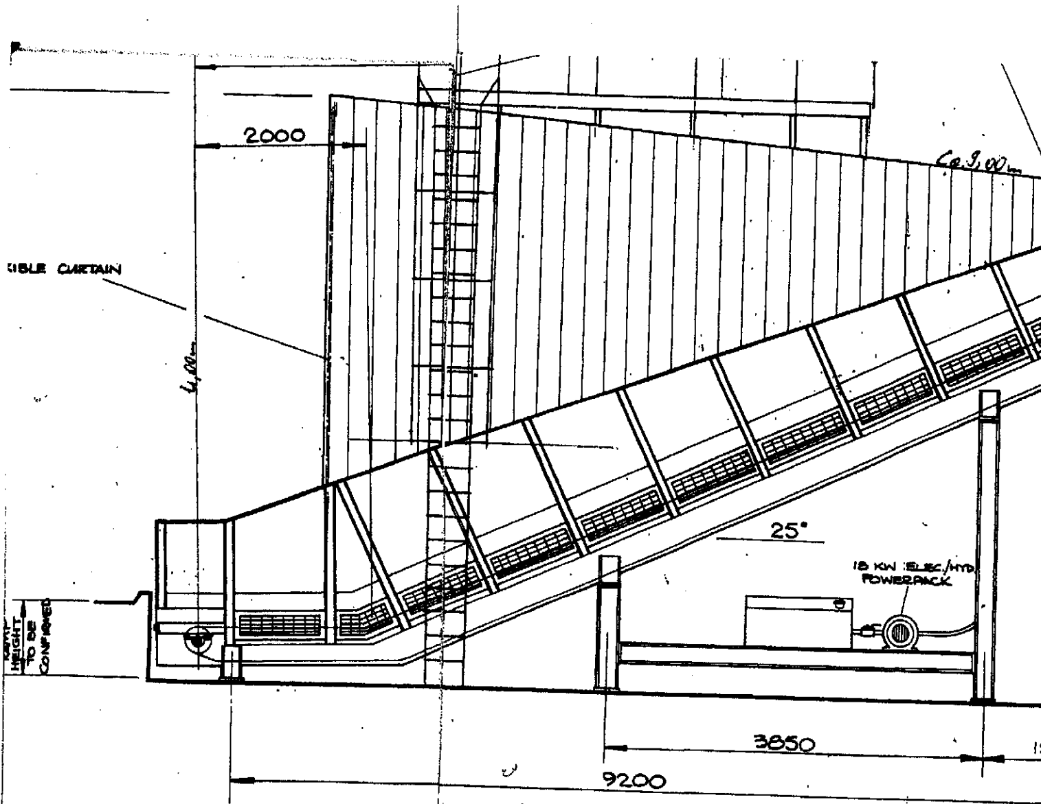
SIDE ELEVATION
